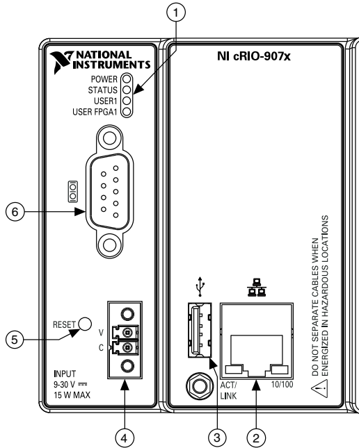
Figure 1. CompactRIO cRIO-9075/9076
