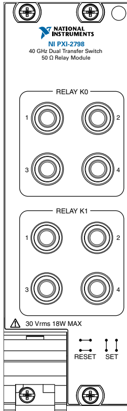
Figure 5. NI 2798 Front Panel
