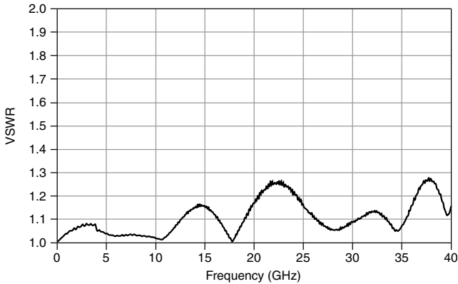
Figure 3. Typical VSWR
