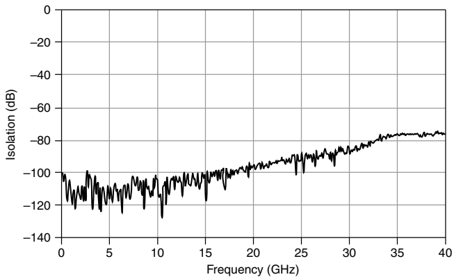
Figure 2. Typical Isolation
