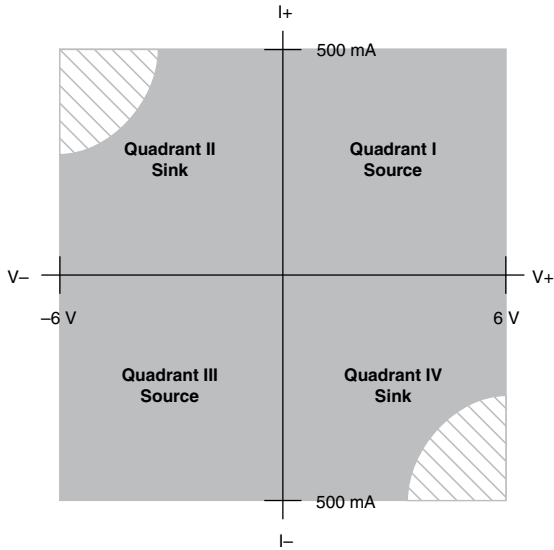
Figure 1. PXle-4144 Quadrant Diagram, All Channels
