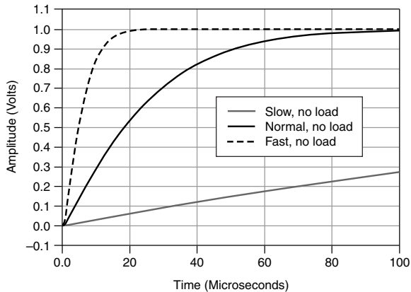
Figure 3. 1 mA Range, No Load Step Response, Nominal
