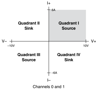
Figure 1. PXIe-4113 Quadrant Diagram
