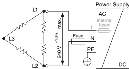
Figure 2-3. NI PS-14 in Two-Phase Operation
