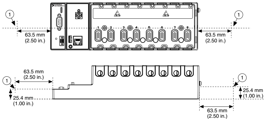
Figure 11. cRIO-9066 Ambient Temperature Location
