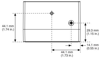
Figure 8. cRIO-9066 Side Dimensions
