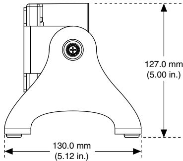
Figure 16. cRIO-9066 Desktop Mounting Side Dimensions
