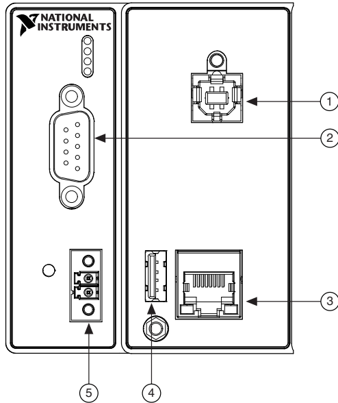
Figure 1. cRIO-9066 Ports and Connectors
