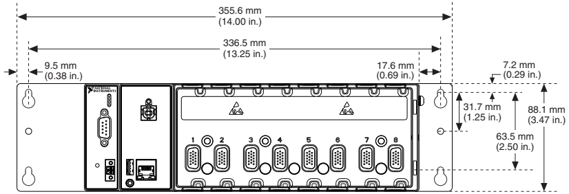
Figure 13. cRIO-9066 Panel Mounting Dimensions
