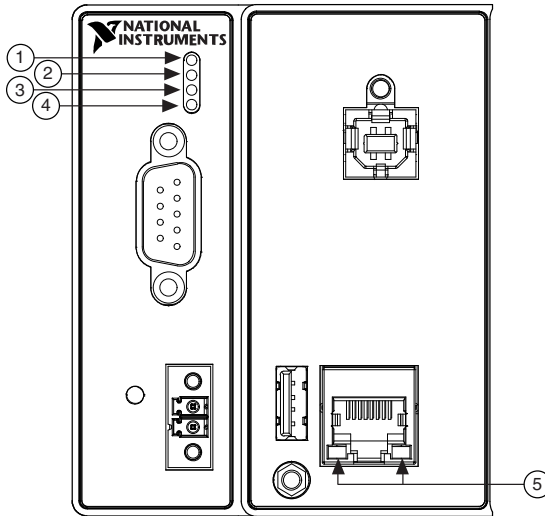
Figure 4. cRIO-9066 LEDs
