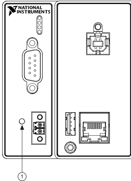
Figure 2. cRIO-9066 Buttons
