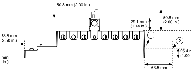
Figure 10. cRIO-9066 Cabling Clearance
