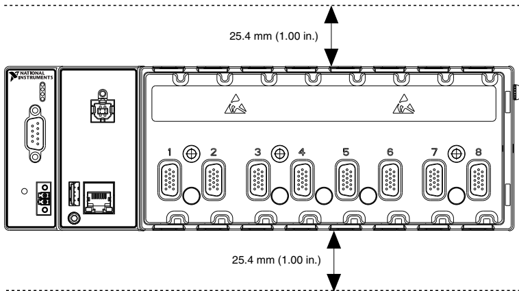
Figure 9. cRIO-9066 Cooling Dimensions
