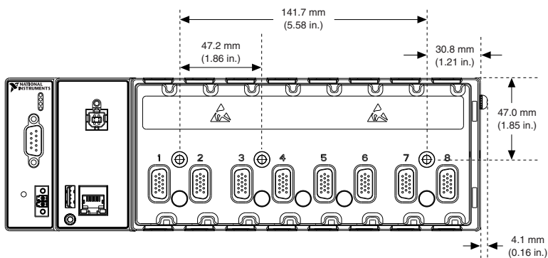
Figure 12. cRIO-9066 Surface Mounting Dimensions
