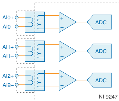
Figure 1. NI 9247 Input Circuitry
