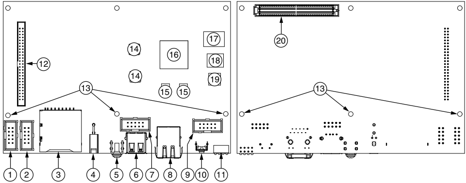
Figure 2. sbRIO-9627 Components
