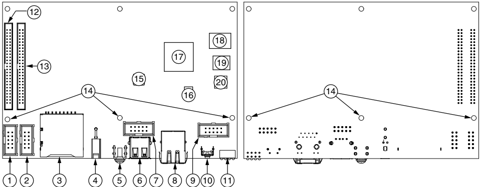
Figure 2. sbRIO-9637 Components
