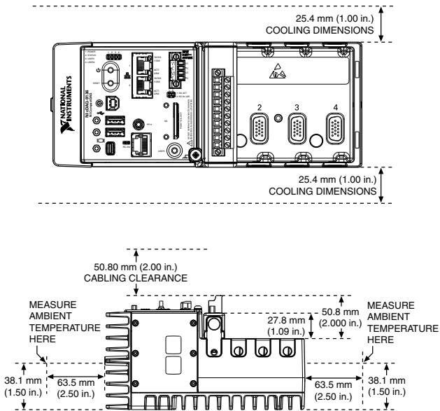
Figure 2. NI cDAQ-9136 Temperature, Cooling, and Cabling Dimensions
