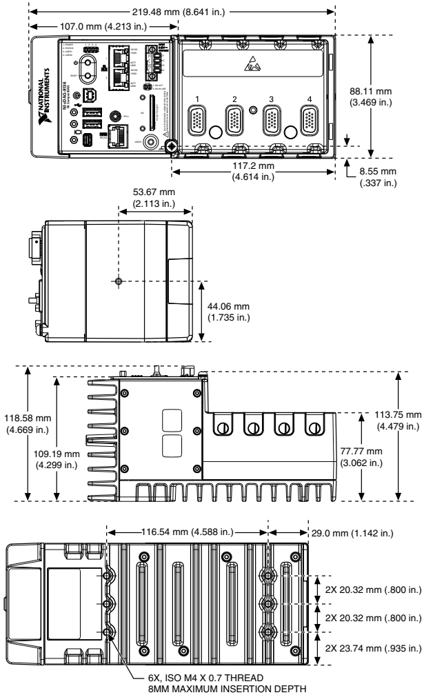
Figure 1. NI cDAQ-9136 Dimensions
