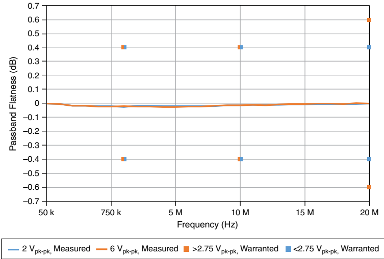
Figure 1. Passband Flatness
