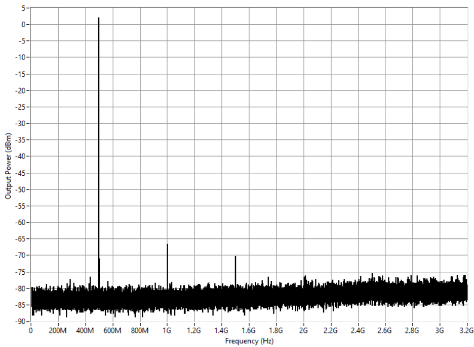
Figure 7. Single Tone Spectrum (Dual Channel Mode, 501 MHz 0 dBFS), Measured [19]
