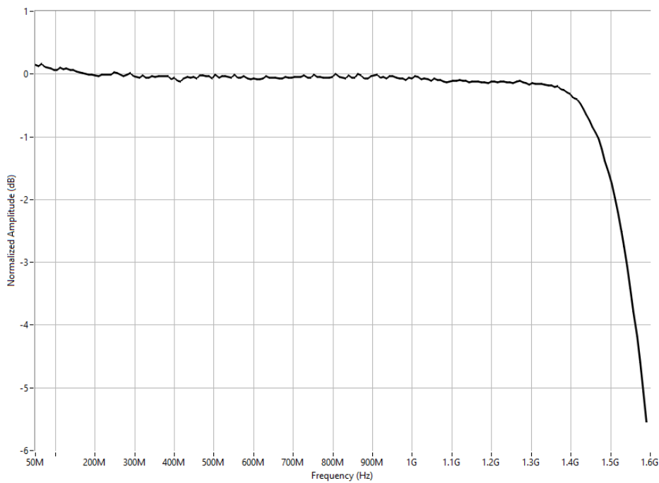
Figure 11. Analog Output Single Channel Mode Frequency Response, No Anti-Image Filter,
