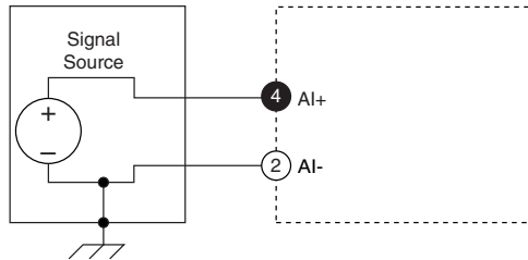
Figure 15. Connecting Grounded Signal Sources to the FieldDAQ Device
