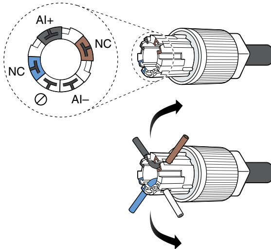
Figure 12. Cable-Side Connections
