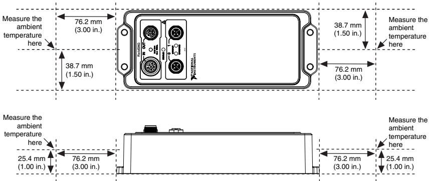
Figure 35. Ambient Temperature Locations, Horizontal Mounting Configuration
