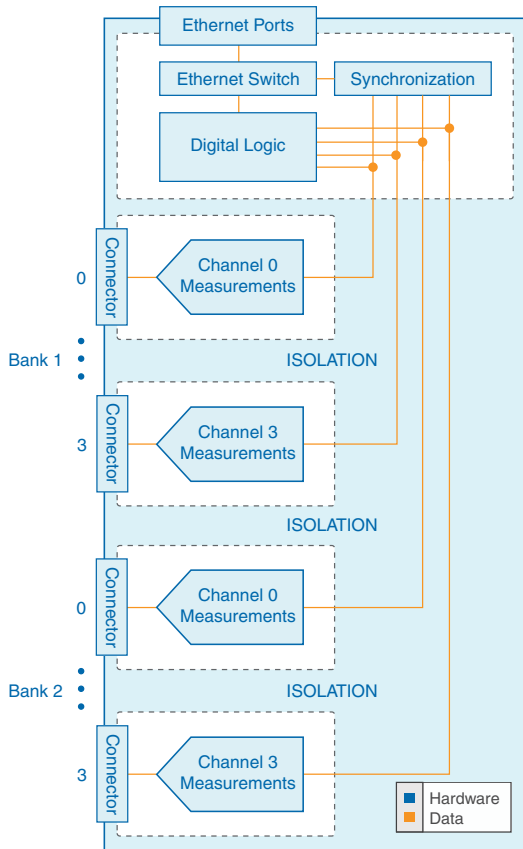
Figure 9. FD-11605 Block Diagram
