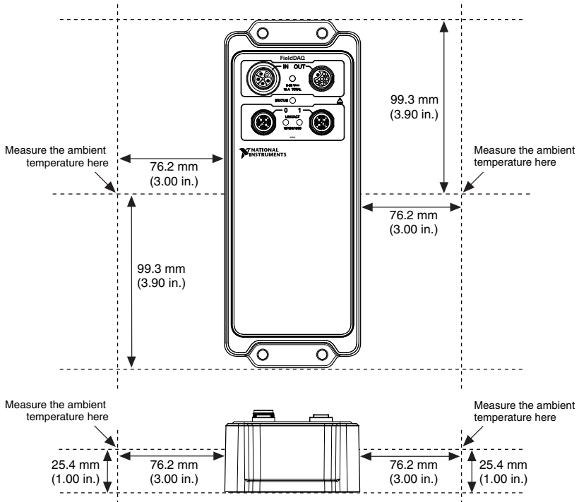
Figure 36. Ambient Temperature Locations, Vertical Mounting Configuration
