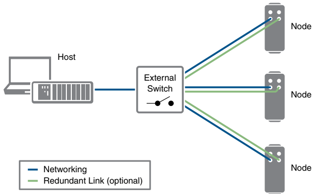
Figure 27. Star Topology
