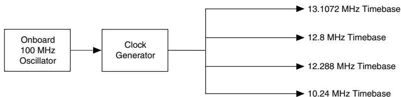
Figure 23. Clock Routing Circuitry
