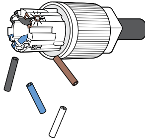
Figure 13. Cutting the Signal Wires
