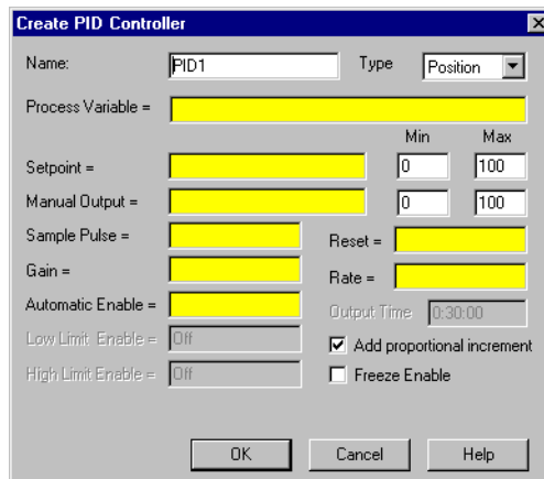
Figure 2-60. PID Definition Parameters Dialog Box
