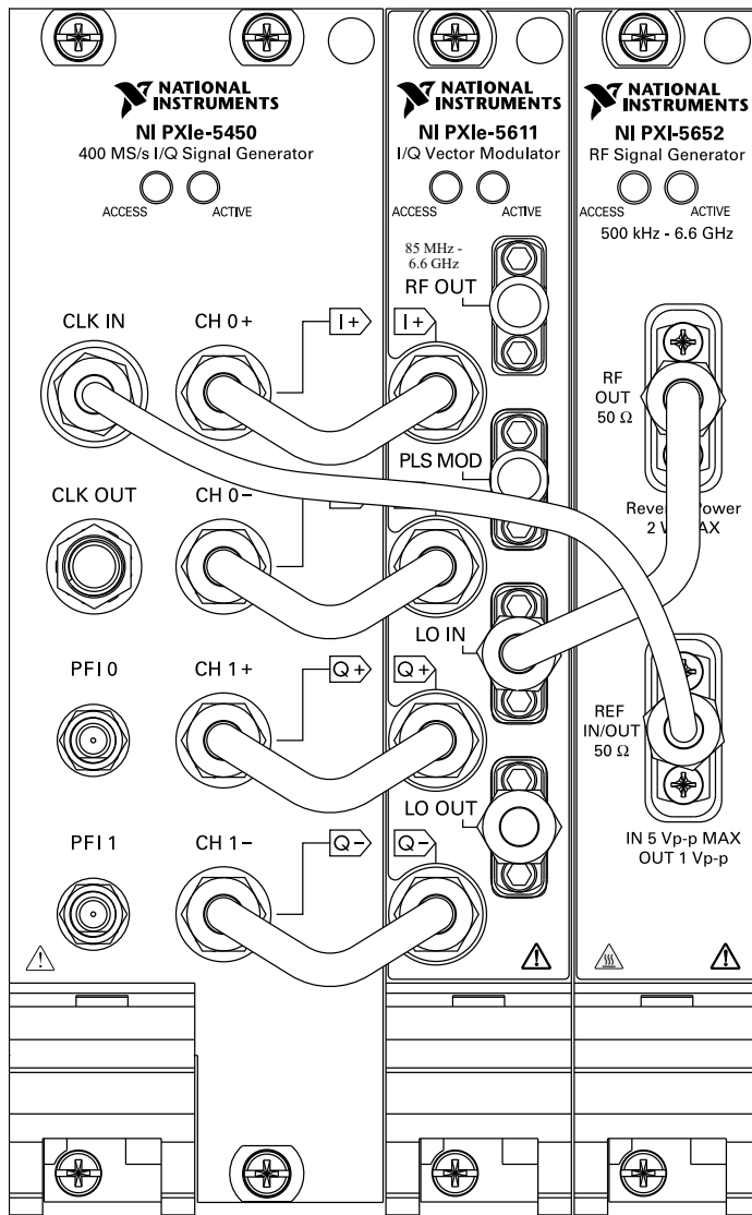
Figure 1. NI 5673 Front Panel
