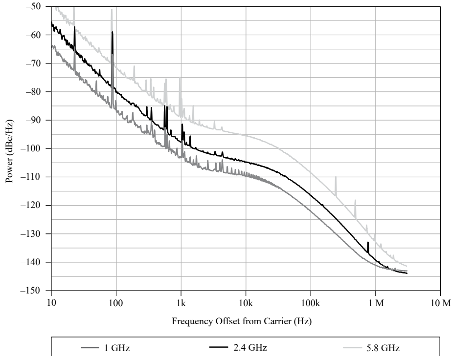
Figure 5. Measured Phase Noise at 5.8 GHz
