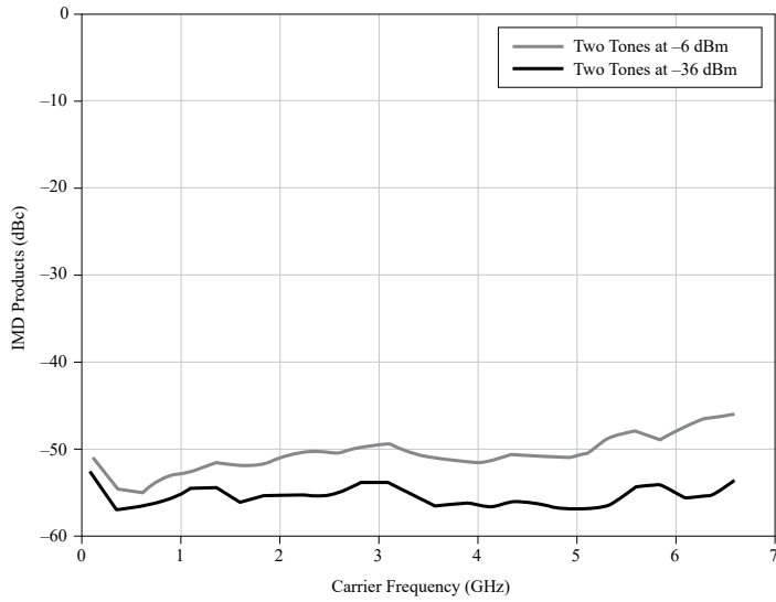
Figure 12. Measured IMD 3 Products
