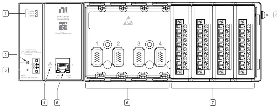
Figure 3. cDAQ-9187 Front Panel
