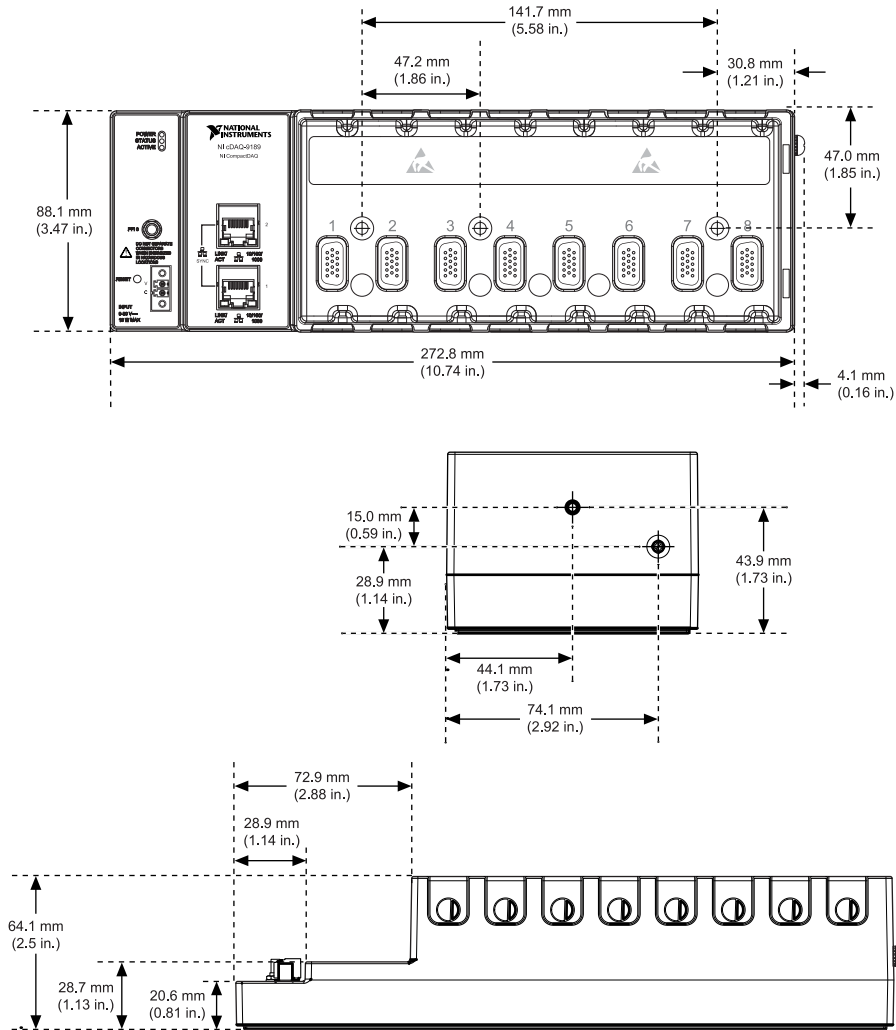
Figure 27. cDAQ-9187 Dimensions
