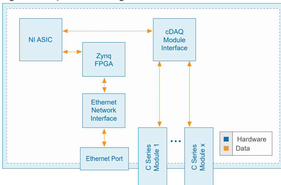
Figure 2. cDAQ-9187 Block Diagram
