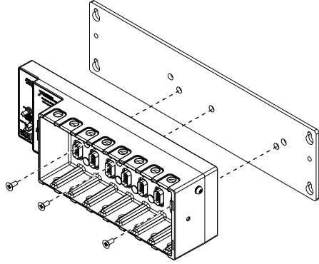
Figure 20. Mounting the Chassis on a Panel (cDAQ-9189 Shown)
