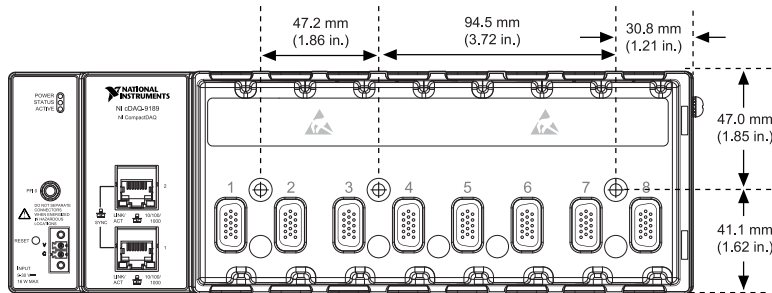
Figure 18. cDAQ-9187 Surface Mounting Dimensions (cDAQ-9189 Shown)
