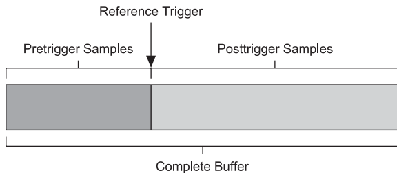
Figure 31. Reference Trigger Final Buffer
