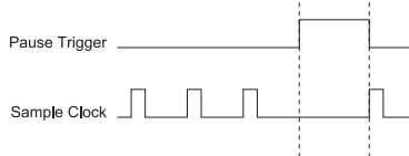
Figure 39. DO Pause Trigger with the Onboard Clock Source
