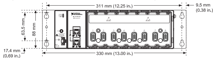
Figure 21. cDAQ-9187 Panel Mounting Dimensions (cDAQ-9189 Shown)
