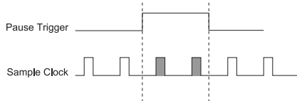
Figure 40. DO Pause Trigger with Other Signal Source
